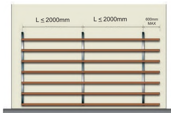
Horizontal Installation
