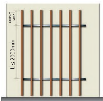
Vertical Installation
